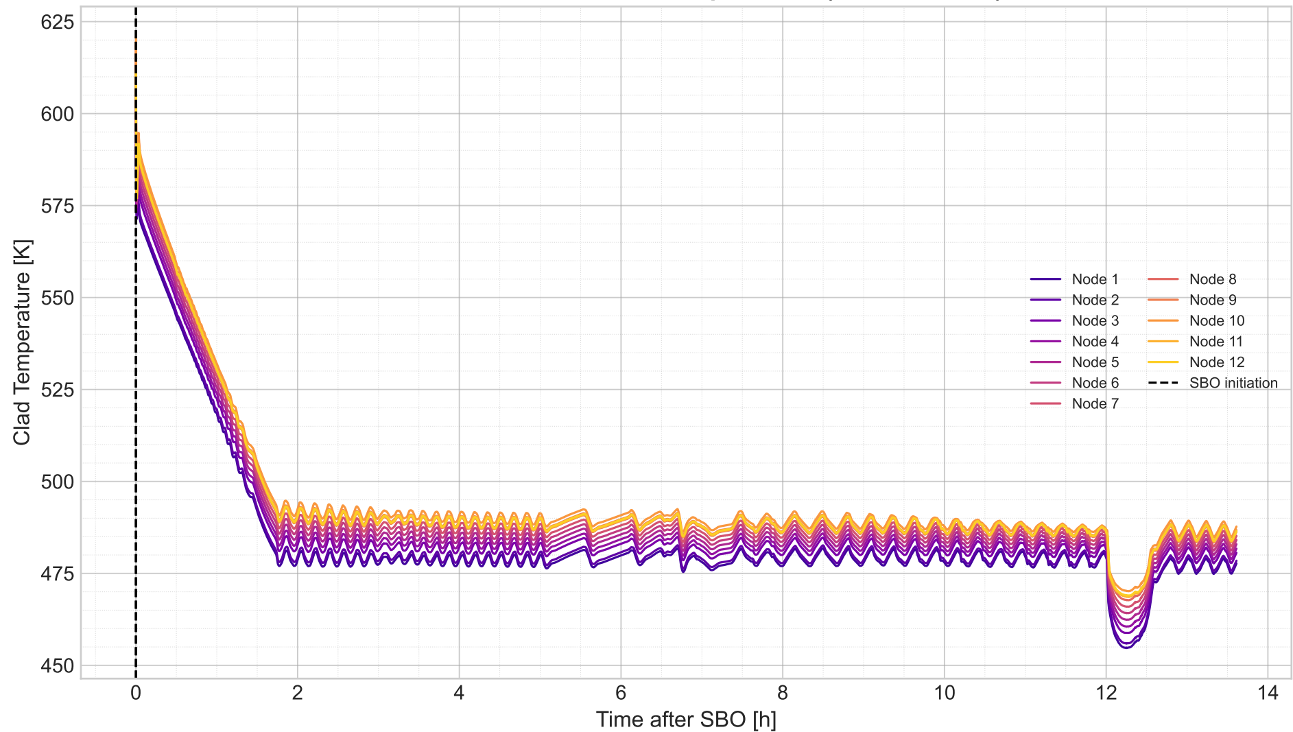
Base Case - Clad Surface Temperatures (all axial nodes)
